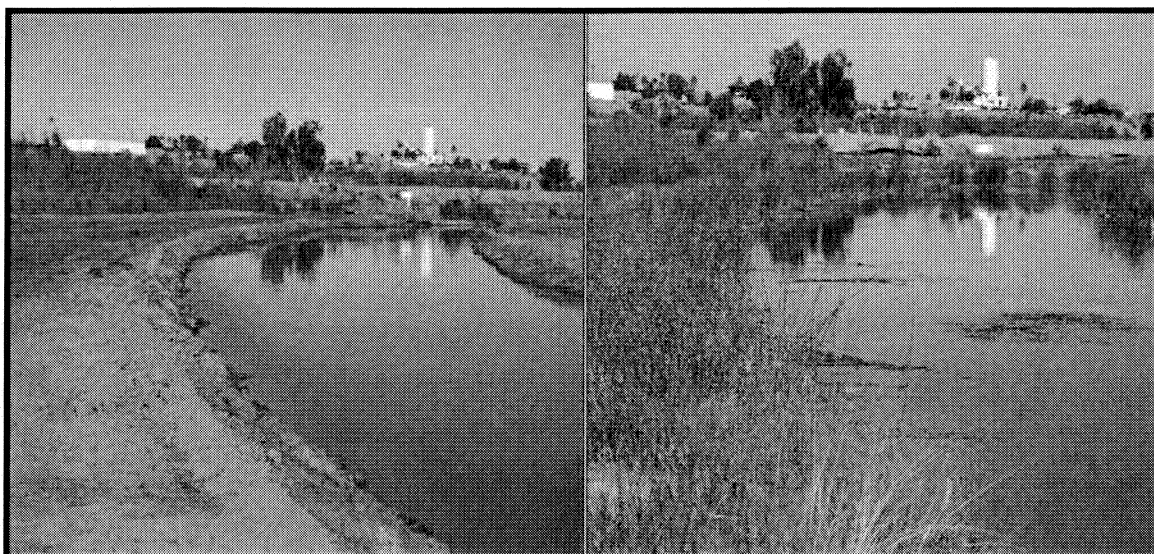
Figure 31. Before and after photos documenting bankline restoration efforts along the South Channel within Yuma East Wetlands. 06-140WPF
