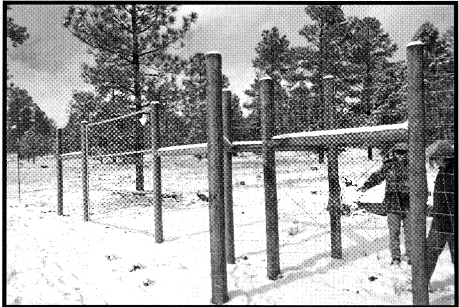
Figure 28. One of five elk proof exclosures constructed by the National Wild Turkey Federation to protect springs and wet meadow habitats in the Apache-Sitgreaves National Forest, Springerville Ranger District. 03-119WPF
